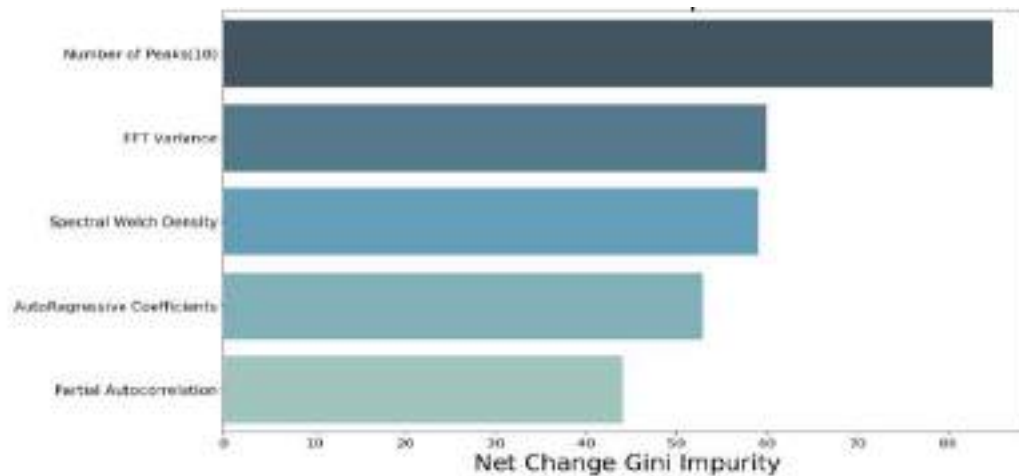
Figure 4. LGBM features
