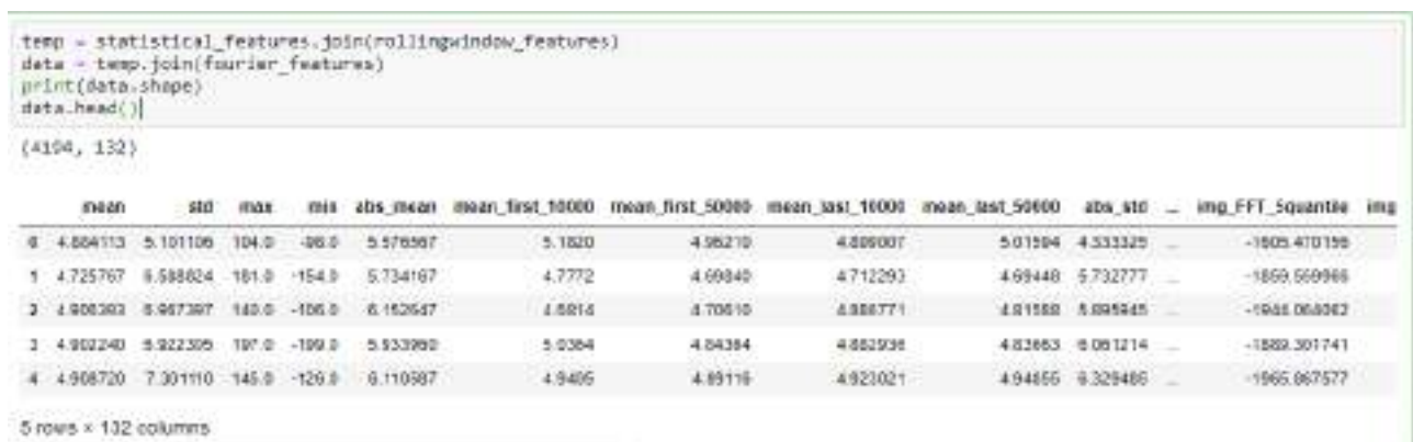
Figure 3. Training data
